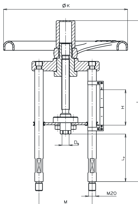
Hand wheels for valves NPS 8" - 16"
