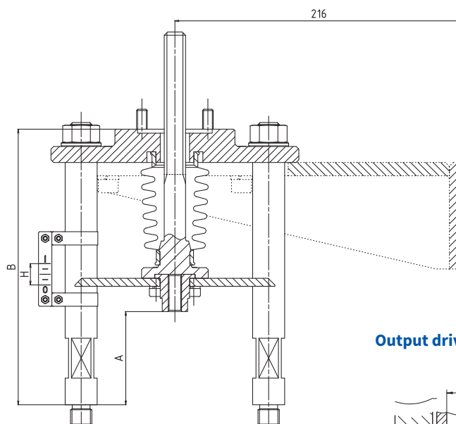
For valves Number of columns A B Weight [kg] CV 2xx NPS 1/2" - 2 1/2" 4 70 207 6 kg (+ 6 kg console) CV 2xx NPS 3" - 6" 4 80 245 8 kg CV 2xx NPS 8" - 10" 4 140 420 15 kg
